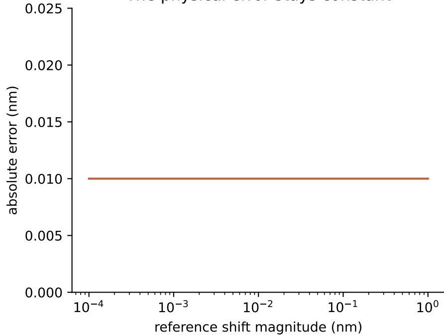
The physical error stays constant
