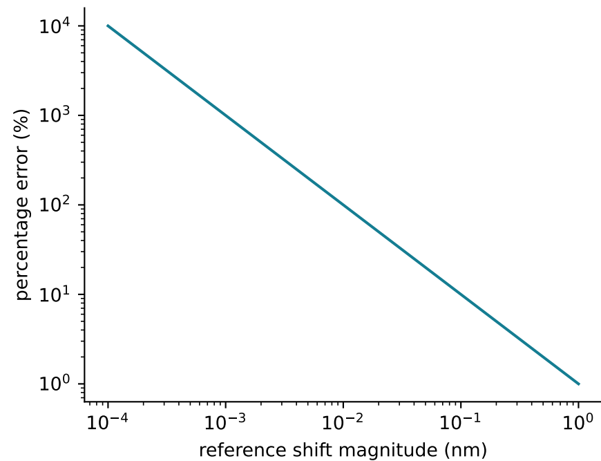
Fixed 0.01 nm error
